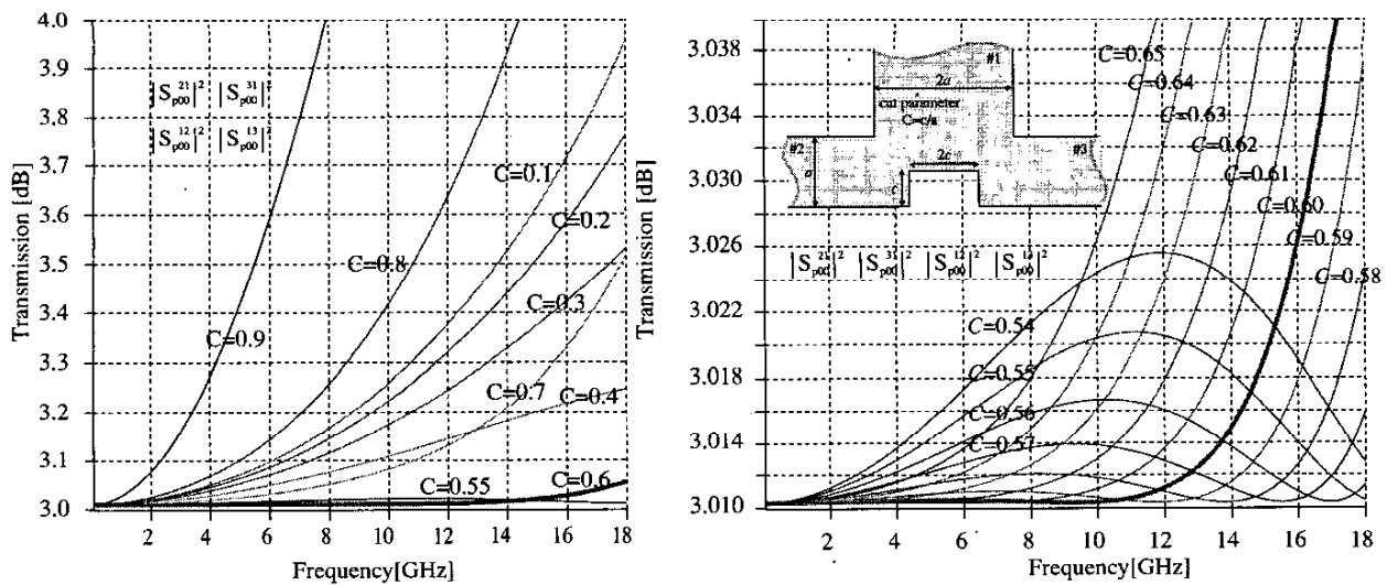
Fig.5 Transmission vs frequency characteristics for planar T-junction with rectangular cut and its detail about C=0.6 (cut parameter C=c/a )
